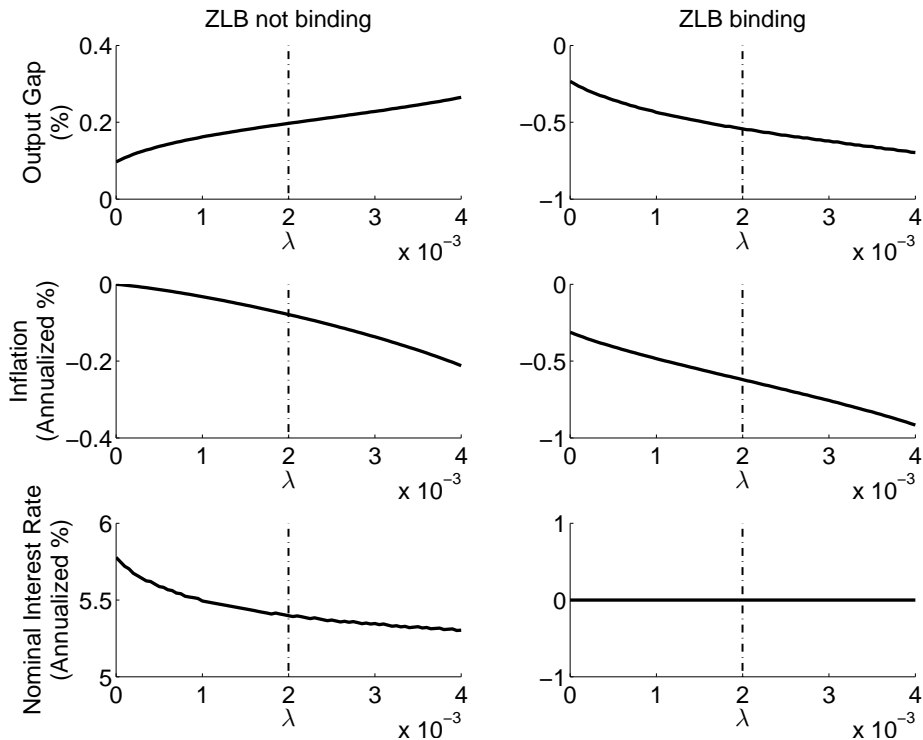
Figure 5: Conditional expectations (Continuous-state model)
