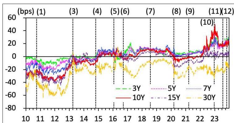
Figure 14: OIS-JGB Spreads
